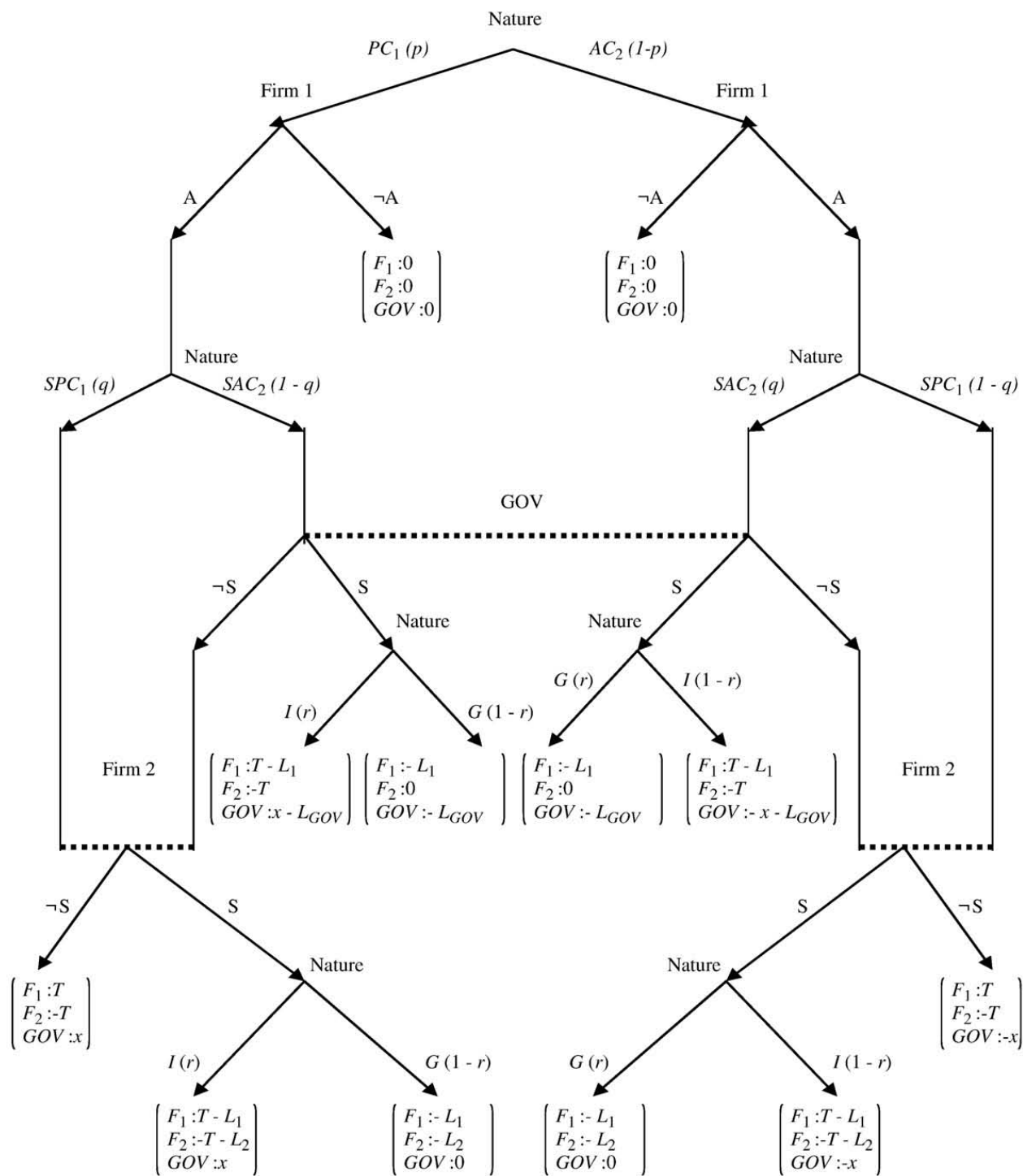
Fig. 1. The game tree with private and public enforcement.
